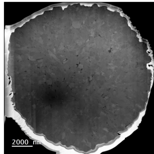
STEM HAADF (High Angle Annular Dark Field)
