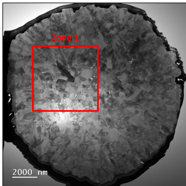
STEM BF (Bright Field)
